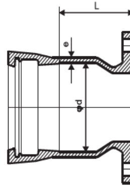
Flange Socket
