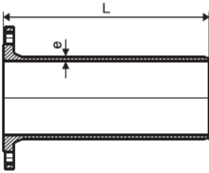
Flange Spigot
